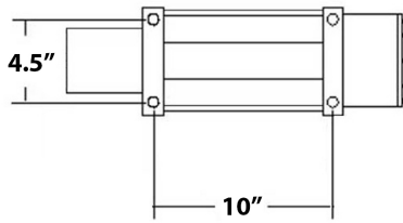
Bolt Pattern
