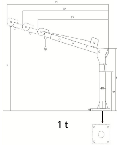
Base Plate 2200lbs Unit: in
