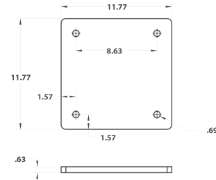
Base Plate 2200lbs Unit: in
