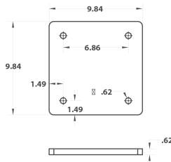
Base Plate 1100lbs Unit: in
