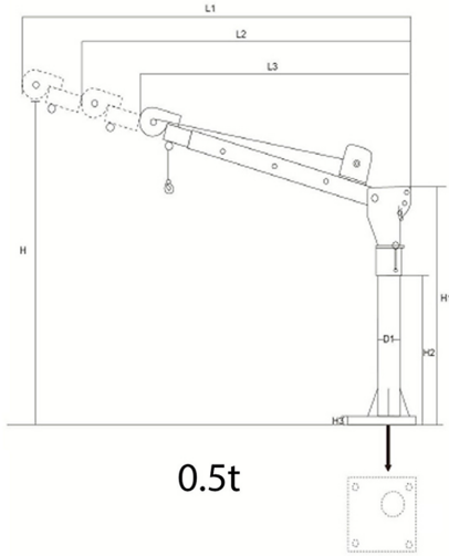
Base Plate 1100lbs Unit: in
