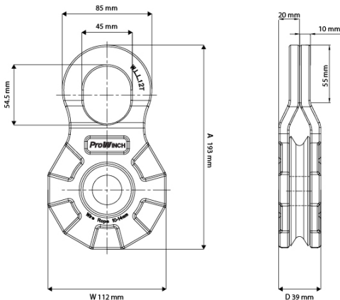
Pulley Housing
