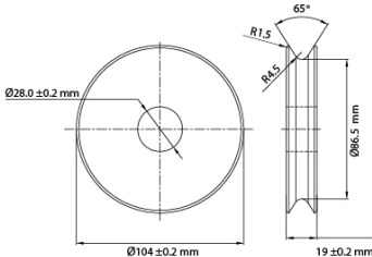
Pulley Disc
